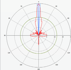
Vertical polarization
